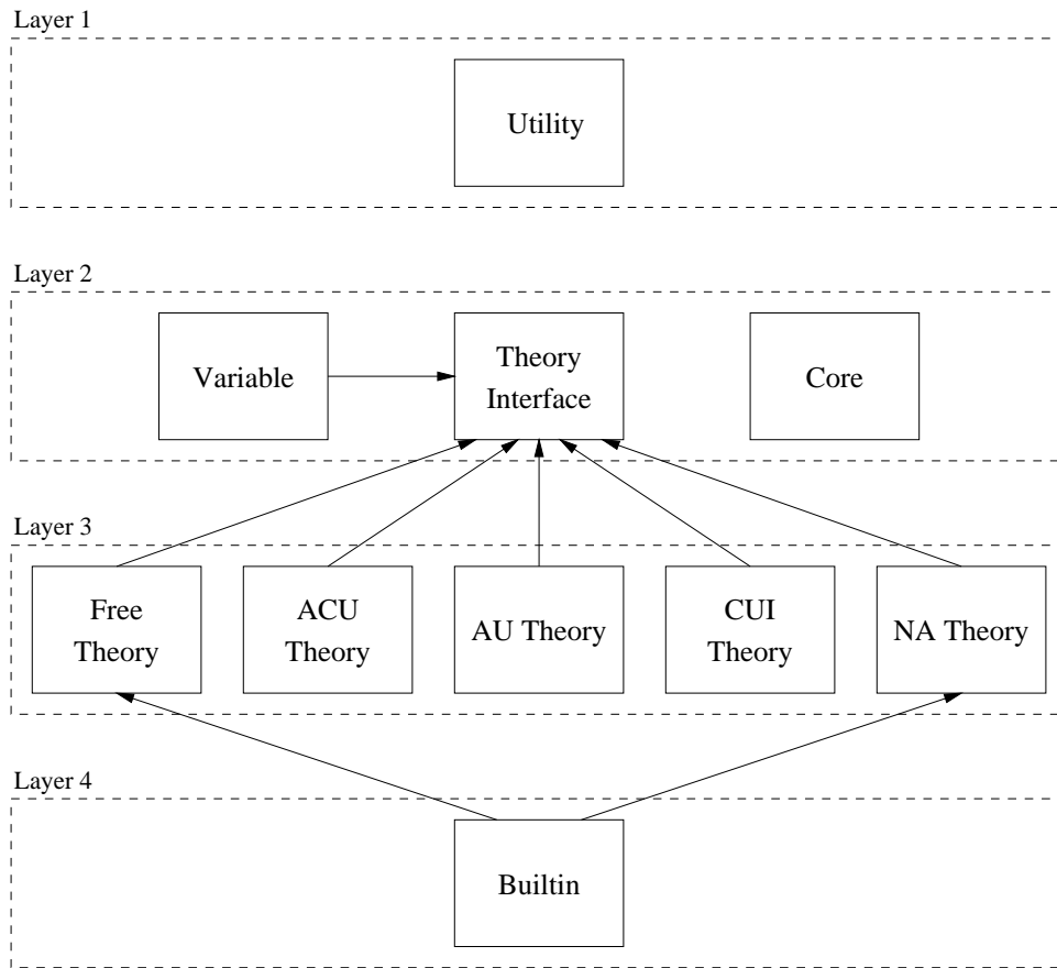
Fig. 2. Architecture of Maude's rewrite engine
